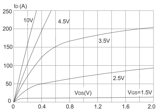
Saturation Characteristics
