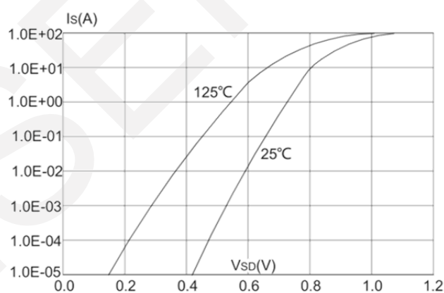
Body-Diode Characteristics
