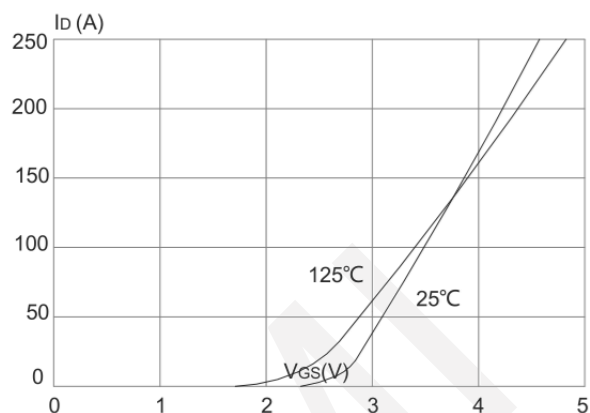
Transfer Characteristics
