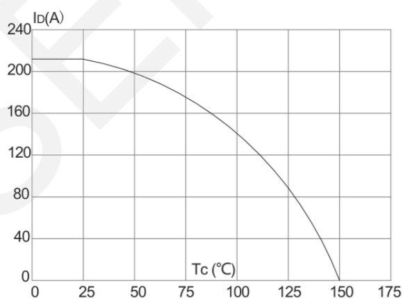
Current De-rating
