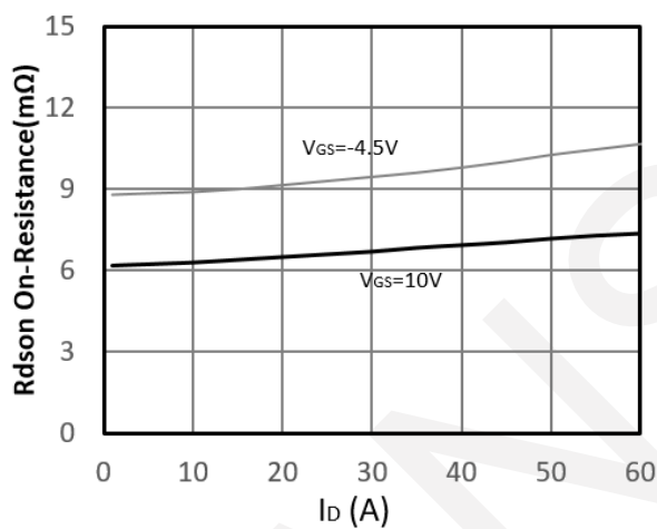
Rdson-Drain Current
