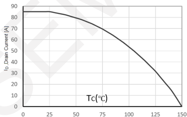
Maximum Continuous Drain Current - Case Temperature
