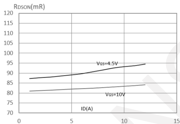
Rdson-Drain Current
