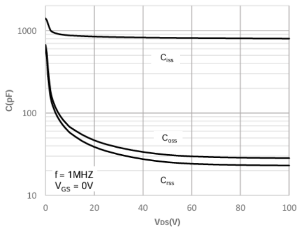
Capacitance - Vds
