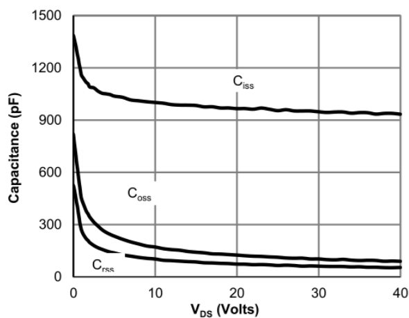
Capacitance Characteristics
