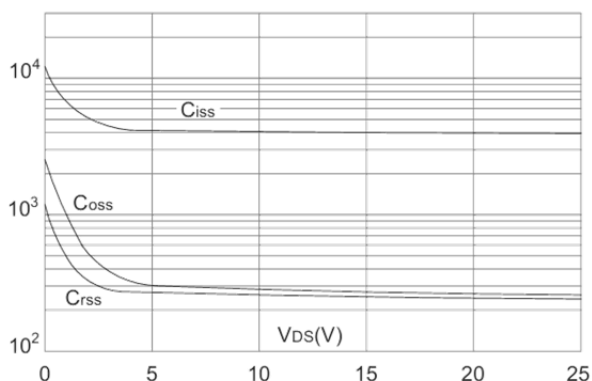
Capacitance Characteristics
