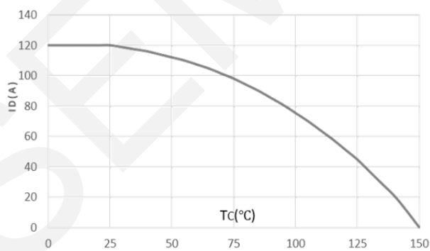
Maximum Continuous Drain Current vs. Case Temperature
