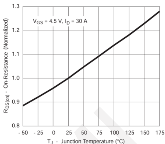
Normalized on Resistance vs. Junction Temperature
