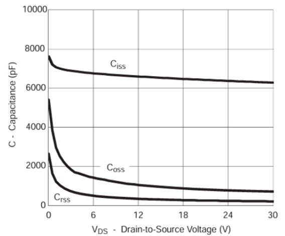
Capacitance Characteristics
