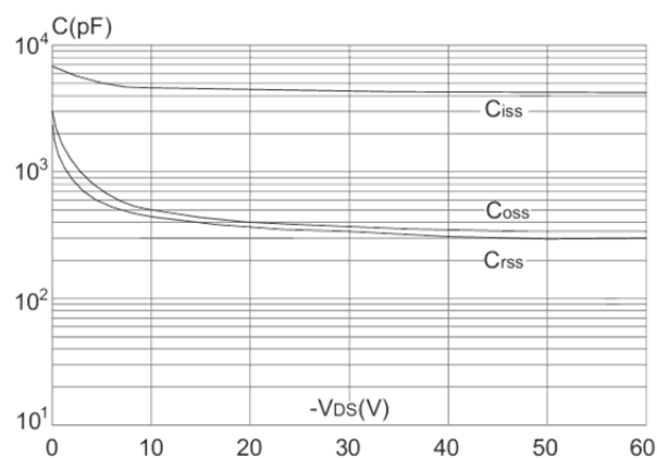
Capacitance Characteristics
