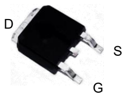
TO-252 Pin Description
