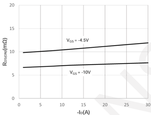
Rdson-Drain Current
