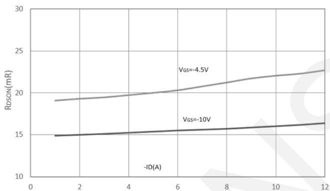
On-resistance vs. Drain Current
