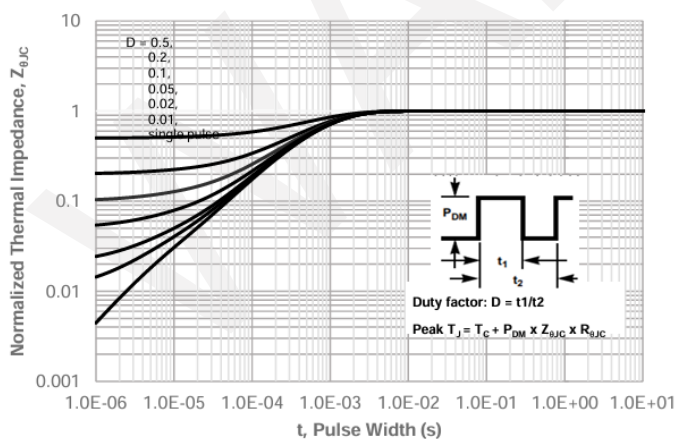
Normalized Maximum Transient Thermal Impedance
