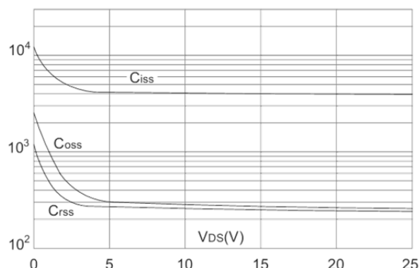
Capacitance Characteristics
