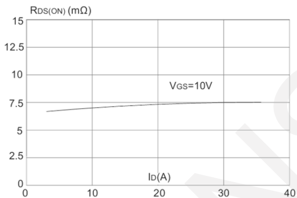
Rdson-Drain Current
