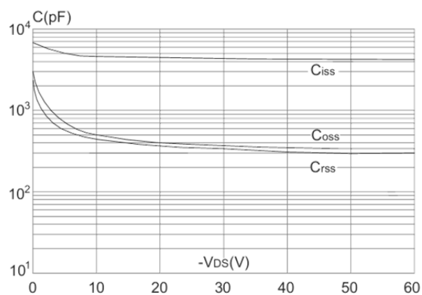
Capacitance Characteristics
