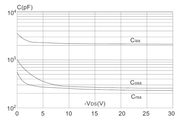
Capacitance Characteristics
