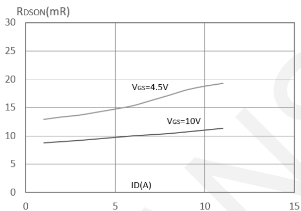
Rdson-Drain Current
