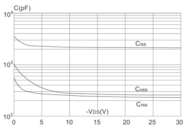
Capacitance Characteristics
