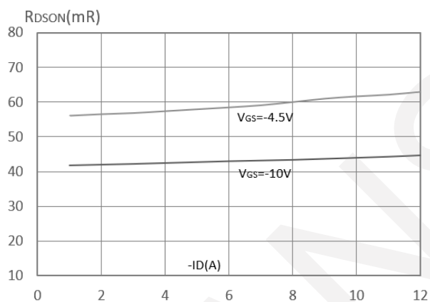
Rdson-Drain Current
