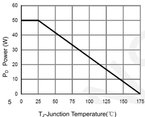
Power De-rating
