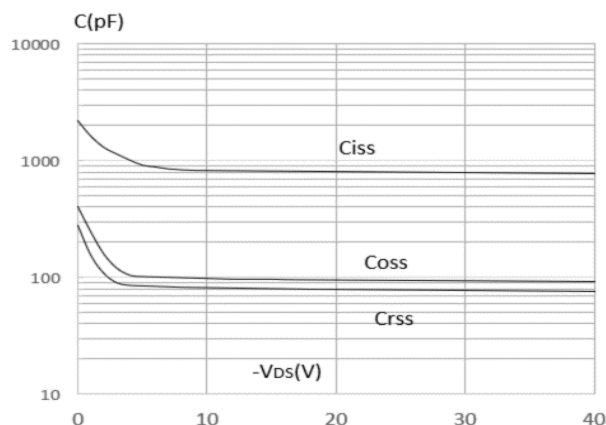
Capacitance Characteristics
