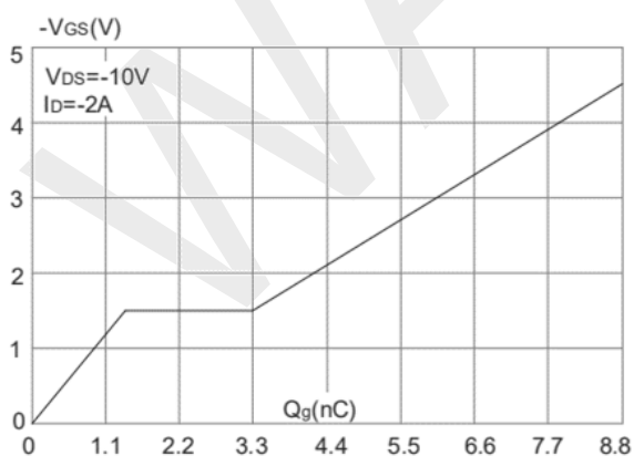
Gate Charge
