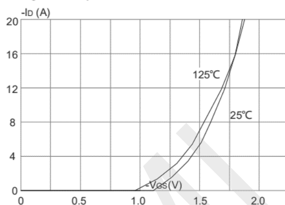
Transfer Characteristics
