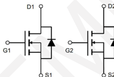
Schematic Diagram
