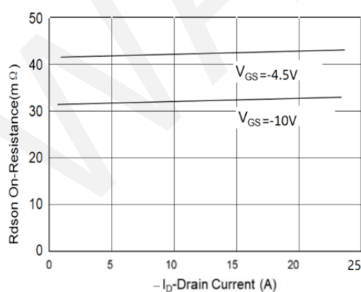
R dson - Drain Current
