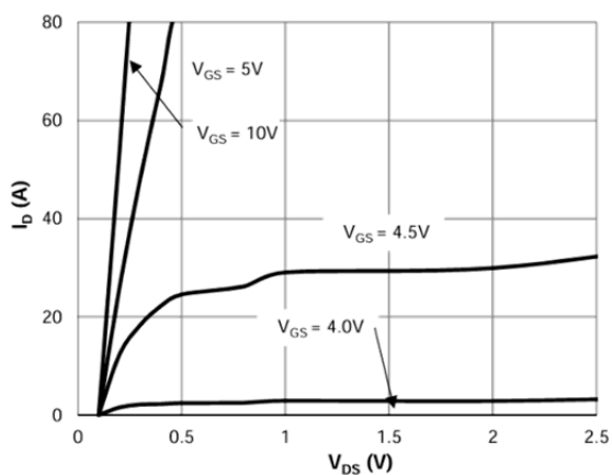
Saturation Characteristics
