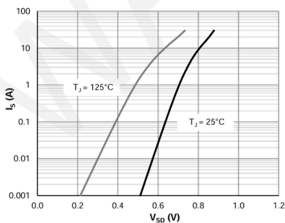
Body-Diode Characteristics
