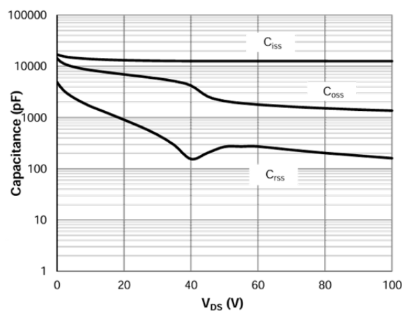
Capacitance Characteristics
