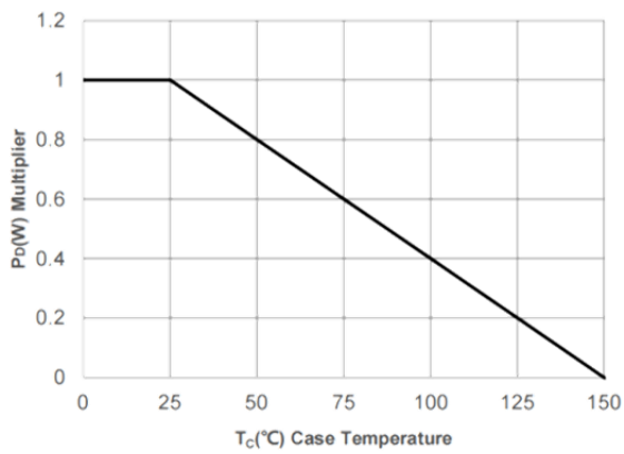
Power De-rating
