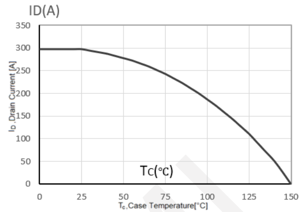
Current De-rating
