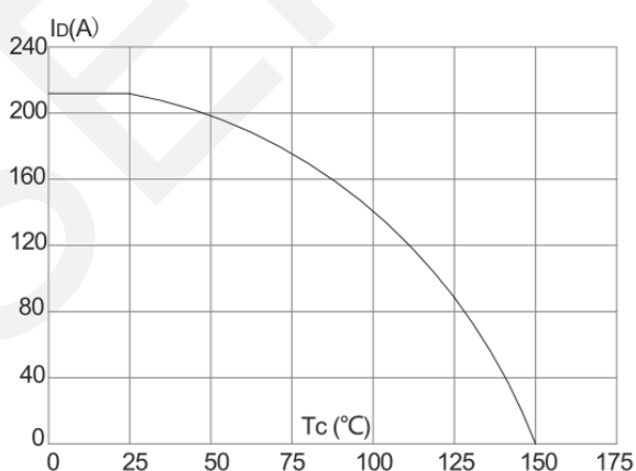
Current De-rating
