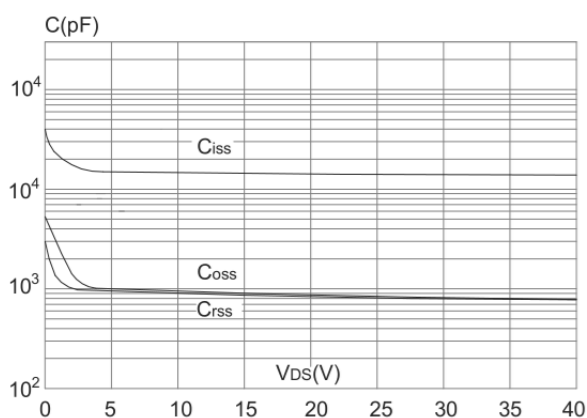
Capacitance Characteristics
