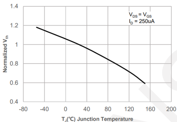
Normalized Threshold Voltage vs. Junction Temperature
