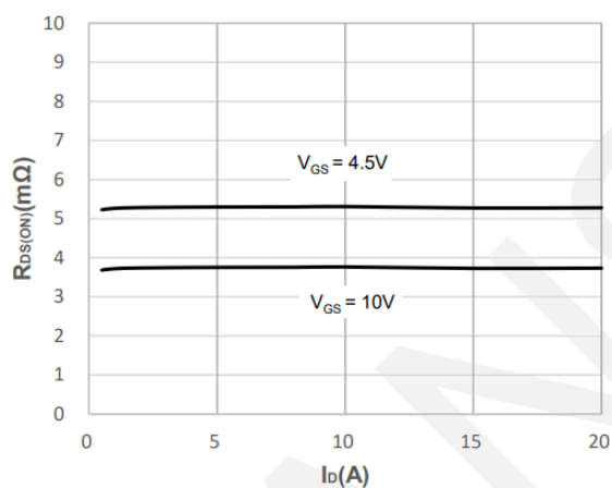
Drain Current
