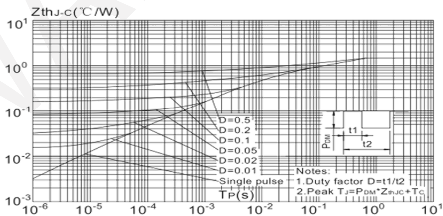
Normalized Maximum Transient Thermal Impedance
