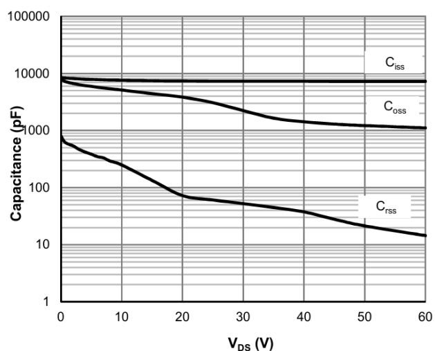
Capacitance Characteristics
