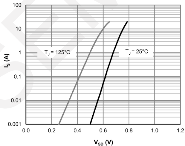
Body-Diode Characteristics
