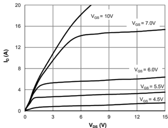
On-Region Characteristics
