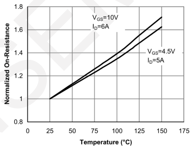
Rdson-Junction Temperature
