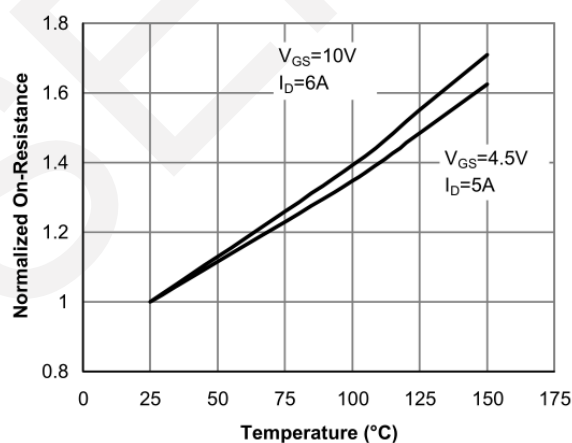
Drain-Source On-Resistance
