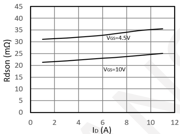
Drain-Source On-Resistance
