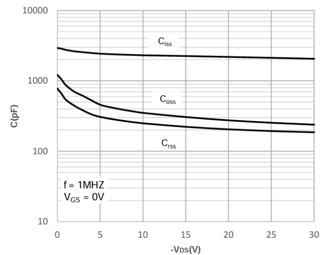
Capacitance Characteristics
