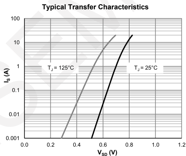
Body Diode Characteristics
