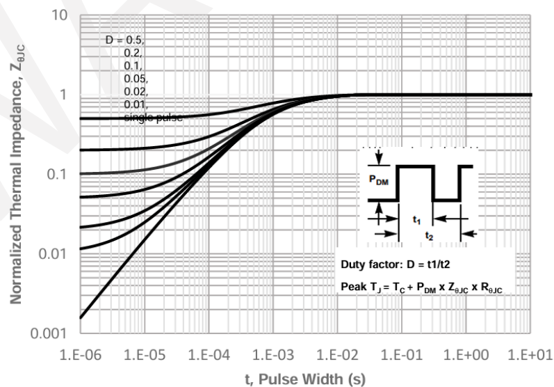
Maximum Effective Transient Thermal Impedance, Junction-to-Case
