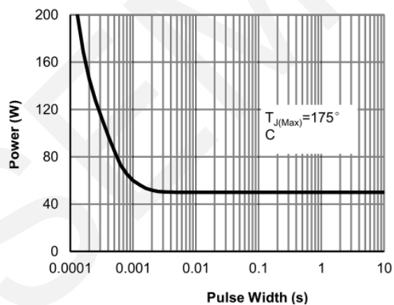
Single Pulse Power Rating
