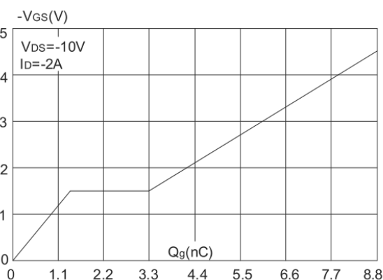
Gate Charge
