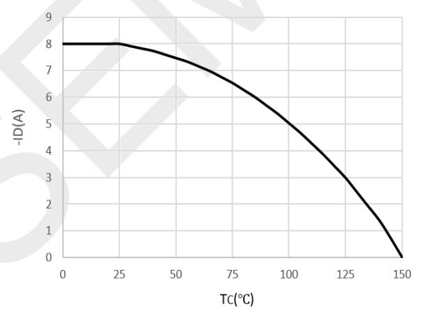
Current De-rating
