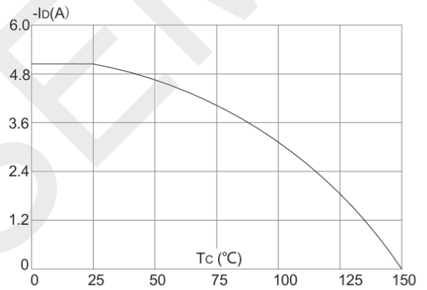
Current De-rating
