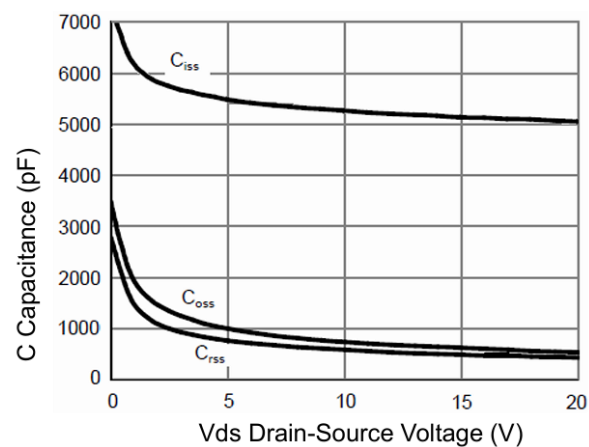
Capacitance Characteristics
