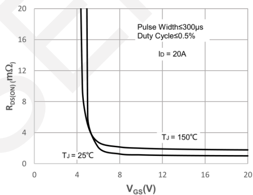
R_{\text{DS(ON)}} vs. V_{\text{GS}}
