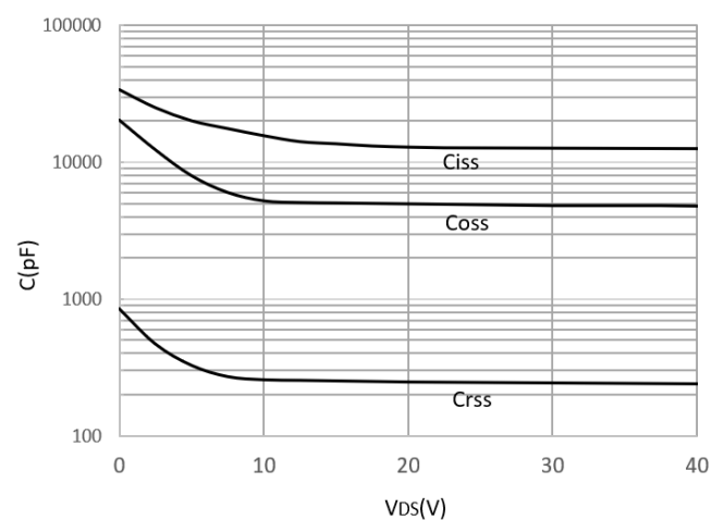
Capacitance Characteristics
