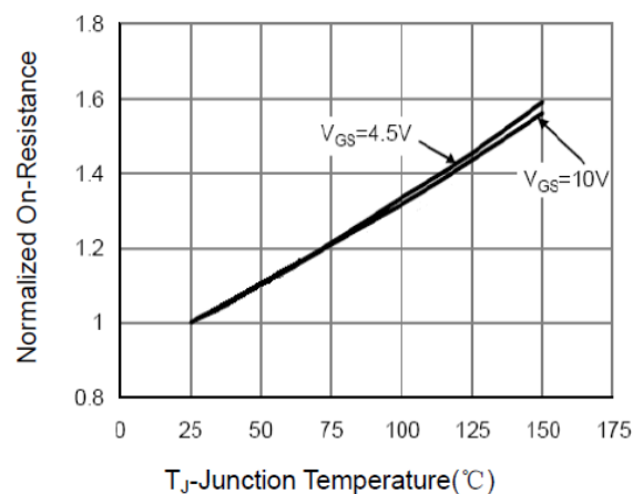
Drain-Source On-Resistance
