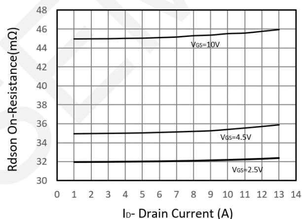
Drain-Source On-Resistance
