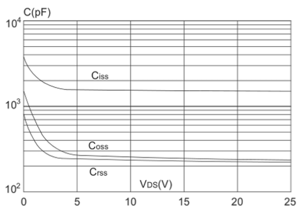
Capacitance Characteristics
