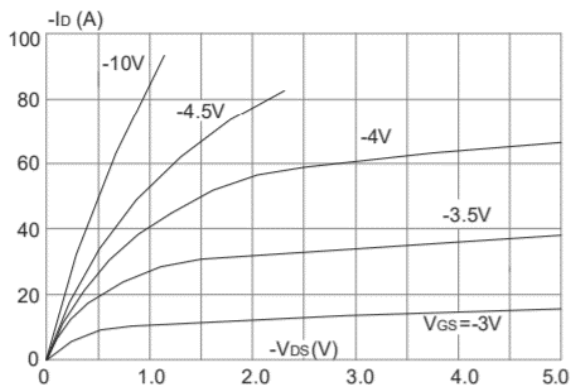
Output Characteristics
