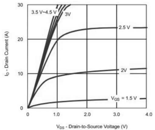
On-Region Characteristics
