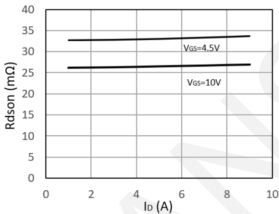
Drain-Source On-Resistance
