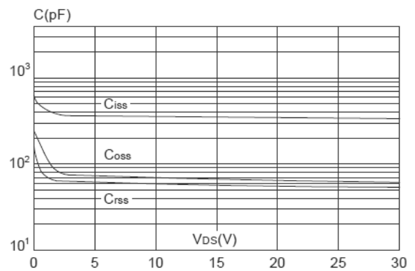
Capacitance Characteristics
