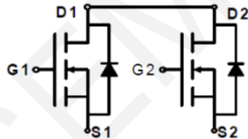
Schematic Diagram
