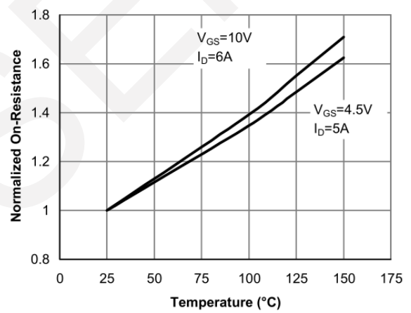
Drain-Source On-Resistance
