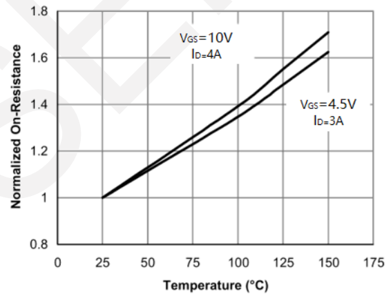
Drain-Source On-Resistance
