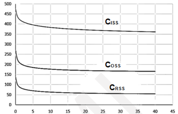
Capacitance vs Vds
