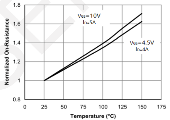
Rdson-Junction Temperature
