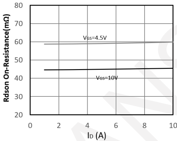
Drain-Source On-Resistance
