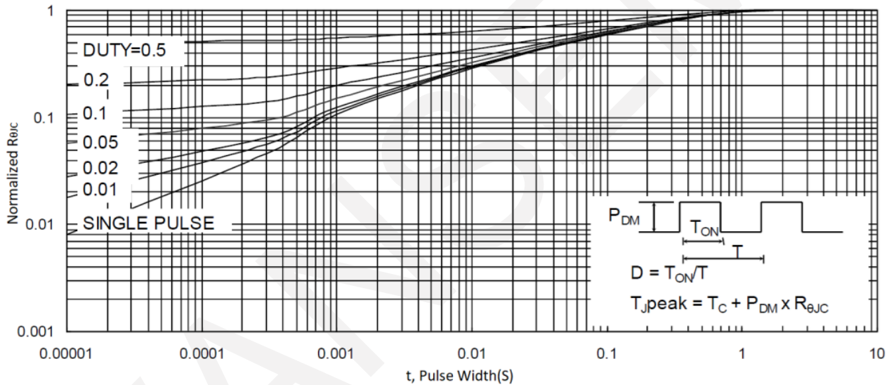
Maximum Effective Transient Thermal Impedance, Junction-to-Case
