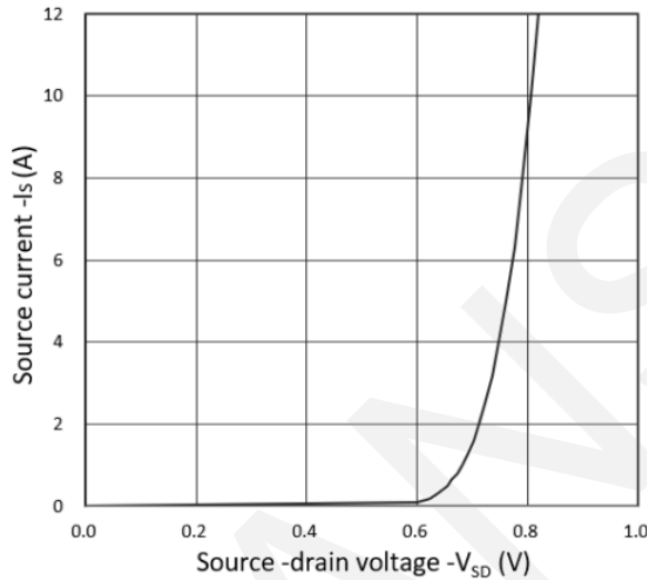
Forward Characteristics of Reverse
