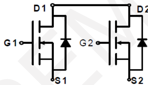
Schematic Diagram
