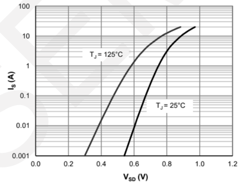
Body Diode Characteristic
