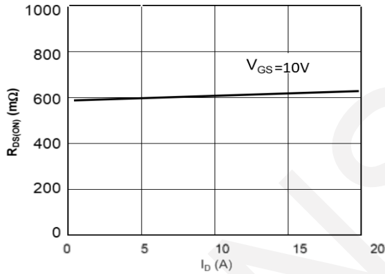
Rdson-Drain Current
